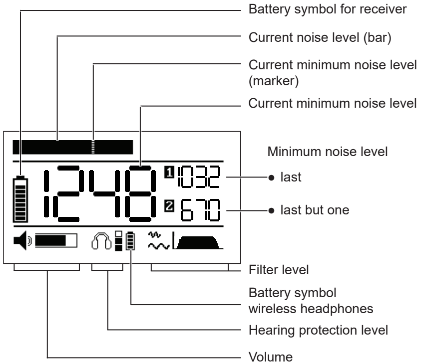
Fig. 2: Display with main view during water leak detection
