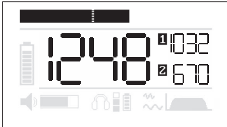
Fig. 5: Graphical and numerical noise level display for water leak detection
