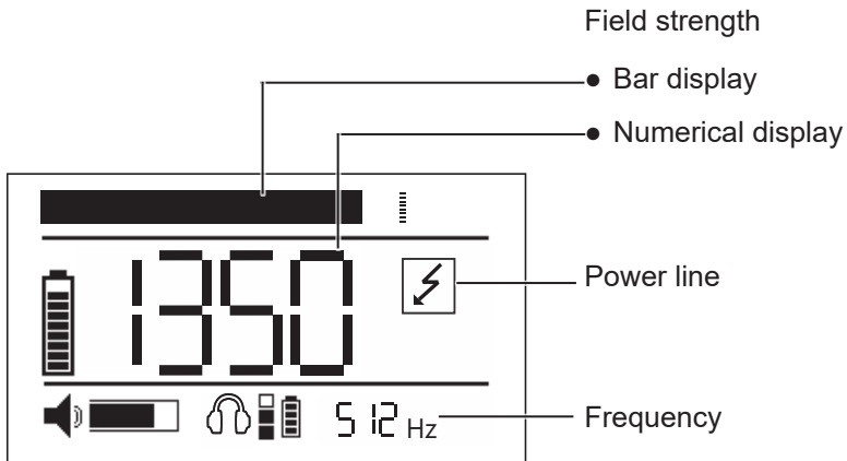
Fig. 3: Display with main view during pipeline location
