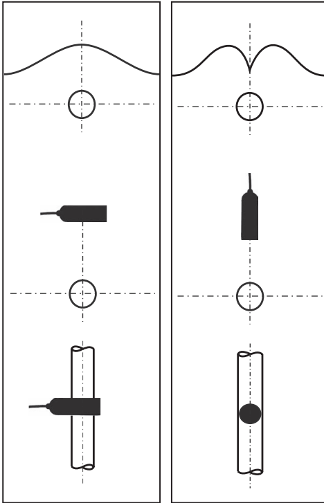
Fig. 13: Signal curve (above) and orientation of the SK 3 search coil over a line
